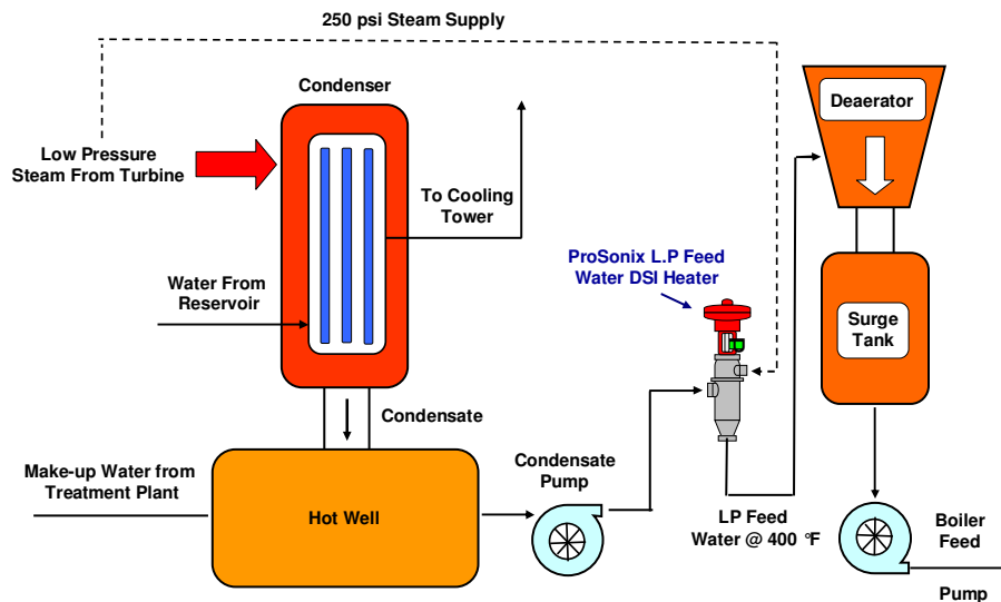
Fig. 1 – Power Plant Feedwater Heater Process diagram
