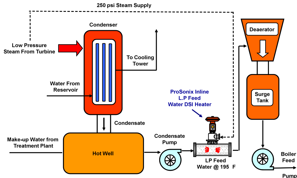
Fig. 1 – Power Plant Feedwater Heater Process diagram
